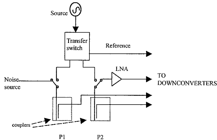
Figure 8. One implementation in which noise figure measurements and S-parameters can be acquired with a single connection of the DUT is shown here. It is important to accurately characterize the path between the noise source and P1 as well as minimize the loss between P2 and the LNA.
