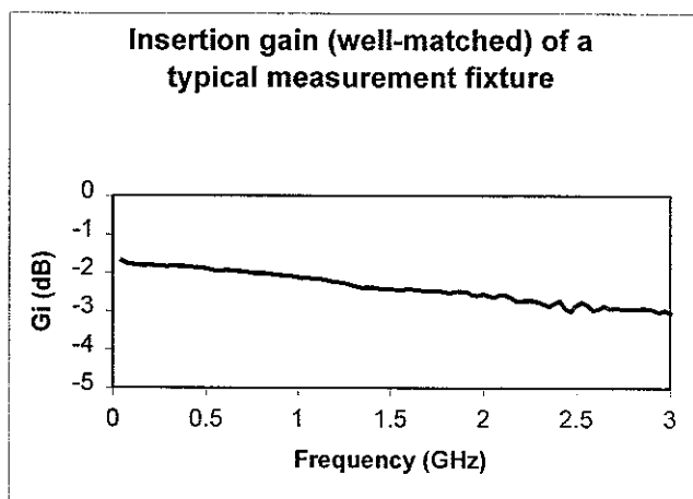
Figure 5. The insertion loss of a typical measurement fixture that may be between the noise source and the DUT is shown here. The frequency response must be taken into account on a broadband measurement.
