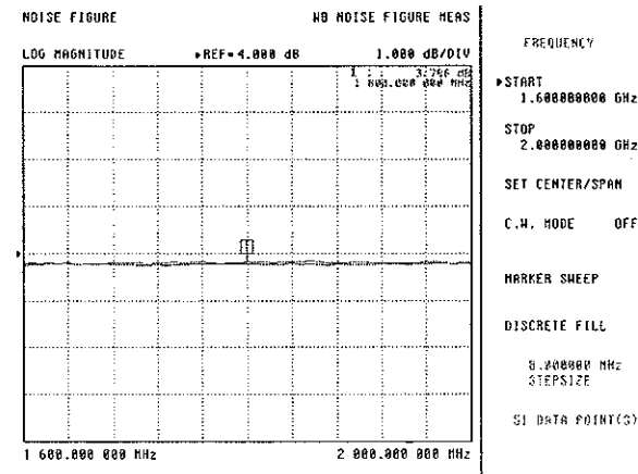
Figure 6. The noise figure of an amplifier without an input network and with an input network (~ 3 dB of loss) and correction applied are shown here. The network's S-parameters were fully characterized and used to compute an ENR correction.
