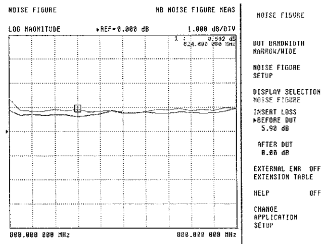
Figure 7. The noise figure of an amplifier without an input network and with an input network and scalar correction applied are shown here. The simple loss-before-DUT correction suffers from lower raw accuracy and neglects match effects, which tend to increase the measurement uncertainty.
