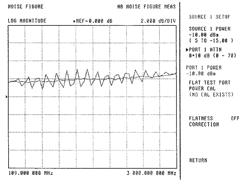
Figure 9. The corrected noise figure of an amplifier when the S-parameter data is acquired at a reasonable power level ( -35 dBm) versus a higher level ( -10 dBm) which is compressing the DUT. Since the higher level represents a different state for the amplifier than when noise data is collected, the results will be erroneous.
