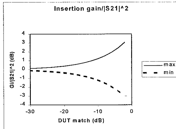
Figure 2. The ratio of insertion gain to |S_{21}|^2 is plotted here as a function of DUT match (assumed symmetric for simplicity). Again the curves show the maximum and minimum values of this ratio as the relative phases vary.
