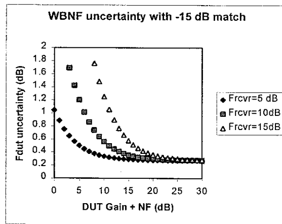
Figure 10. An example uncertainty curve set for wideband noise figure measurements at a DUT match of -15 dB is shown in this figure. Most amplifier measurements will reside in the asymptote of the curves at the right side.
