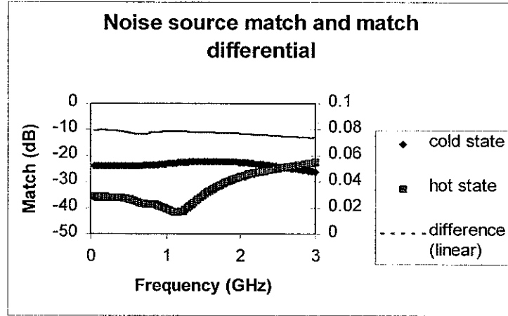
Figure 3. The output match of a commercial noise source is plotted here (both states) along with the vector difference of these matches (upper curve plotted in linear terms against the right axis). The difference is fairly substantial.
